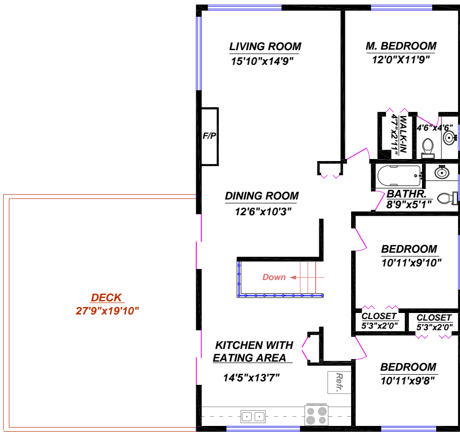
MAIN FLOOR
