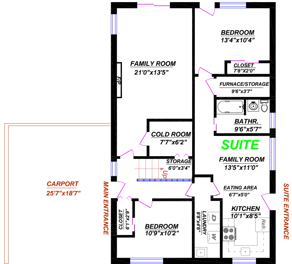
LOWER LEVEL
