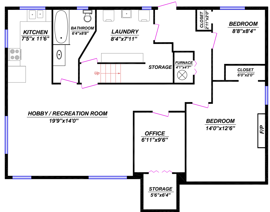
BASEMENT
